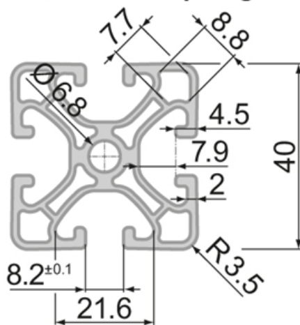
Profile 40 Superlight
