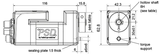
PSD 413-8H (hollow shaft, 3 Nm)
