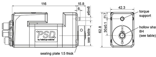
PSD 411-8H (hollow shaft, 1 Nm)
